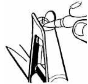
Figure 9-3. Front Sight Adjustment.
